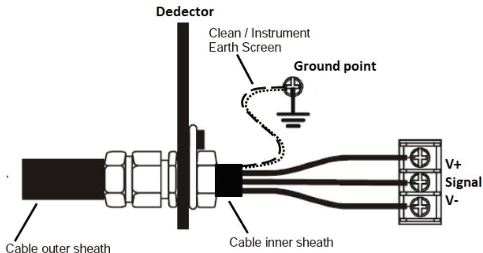
Diagram 8: Grounding
