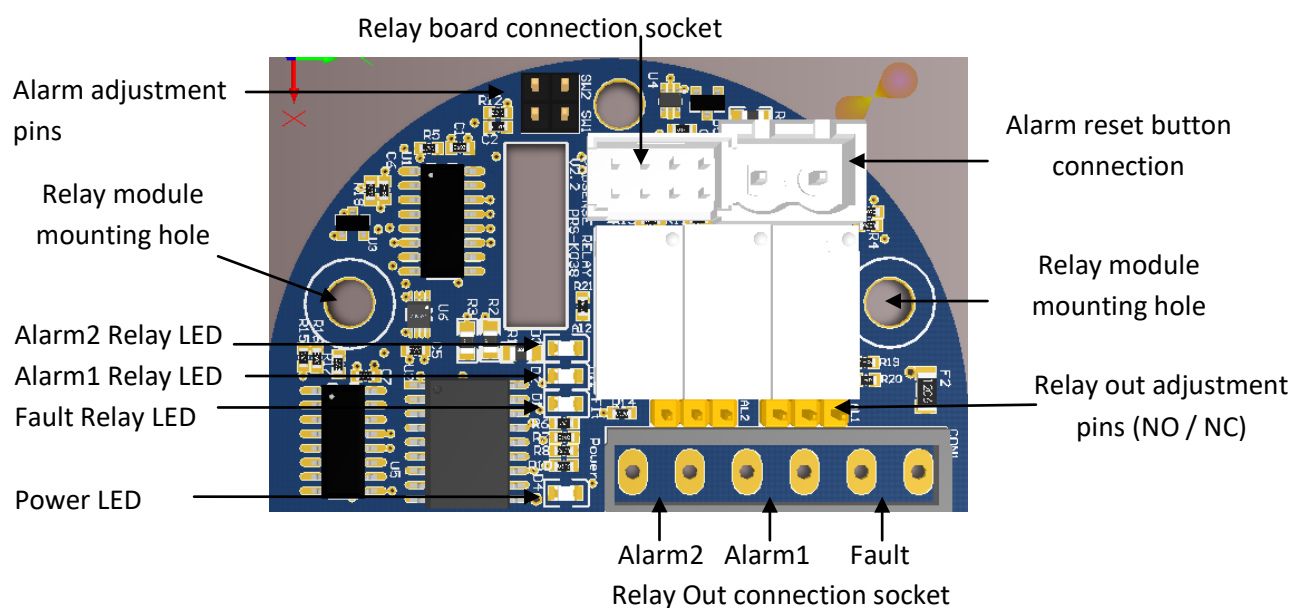
Diagram 14: Relay module
